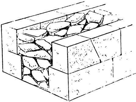
FIG. 70.—Double-faced wall.
